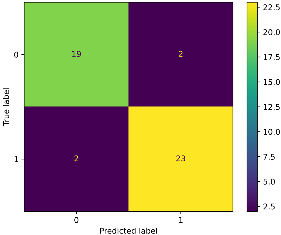
Confusion Matrix for Tuned Random Forest Model
